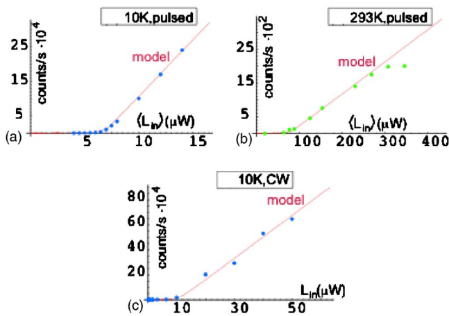
FIG. 2. (Color online) LL curves. (a) Low-temperature lasing (10 K) with pulsed excitation (3.5 ps, 13 ns repetition) shows an averaged threshold of 6.5 \mu\text{W} , corresponding to 21 mW peak power. (b) At room temperature, lasing threshold increases to an averaged 68 \mu\text{W} (221 mW peak). (c) Continuous-wave lasing at low temperature shows a very low threshold of 9 \mu\text{W} . Pump powers are measured before the objective lens.
